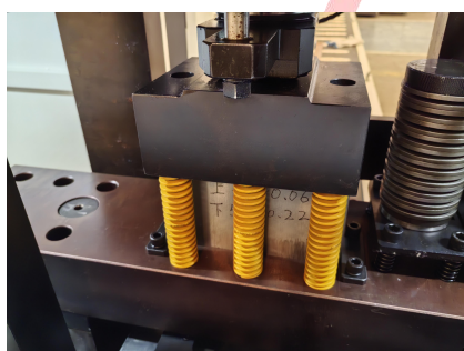
Shearing Mold
